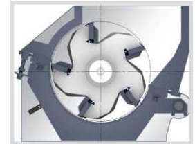
Two Fixed plus Five Rotating Blades
